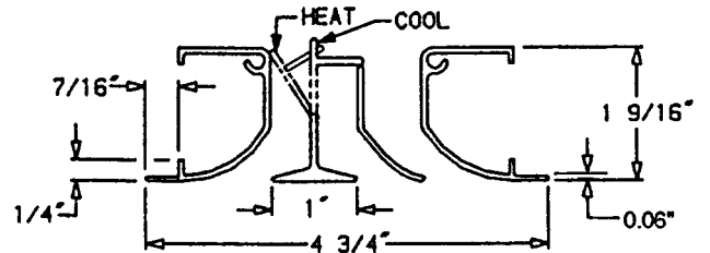
STANDARD EXTRUDED ALUMINUM DM 3-SLOT DIRECTOR DIFFUSER FOR ALL LENGTHS
